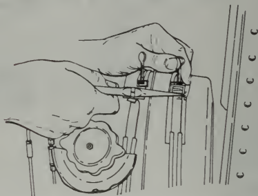
FIGURE 6-15. Removal of securing straps.
